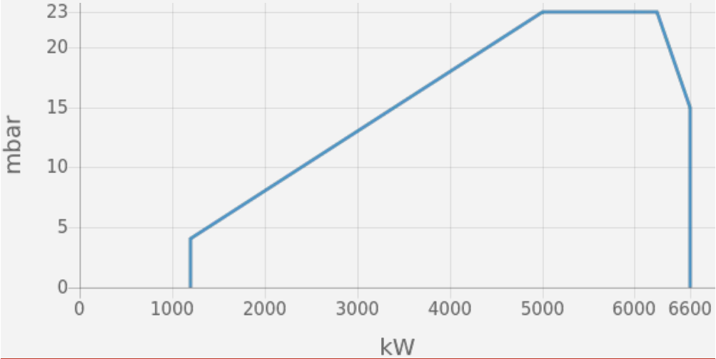
WORKING DIAGRAM
