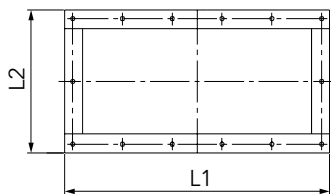
Air connection flange
