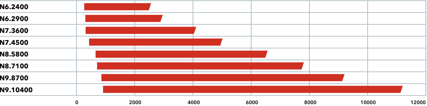
/ GAS RANGE 340 / 11200 kW
