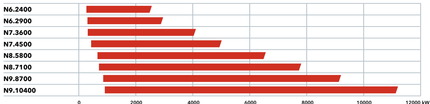
/ LOW NO x up to 10200 kW
