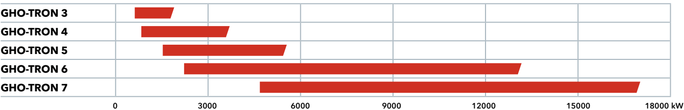
/ DUAL FUEL (GAS/HEAVY OIL) RANGE 414 / 17000 kW
