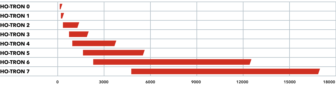
/ HEAVY OIL RANGE 68 / 17000 kW
