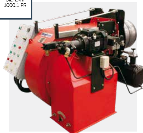
OILFLAM 1000.1 PR Two stage progressive mechanical 3300 - 10500 kW
